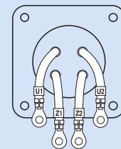
Connection Diagram
