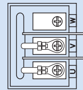
Connection Diagram
